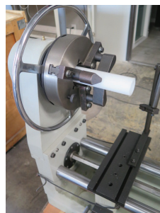
Import 65mm Glass Blowing Lathe w/ 65mm Thru Spindle Bores, 23" (Over Table) x 43 1/2", 0-187 RPM, Stepper Motor and Controller, 8" Chucks, 110 Volts
