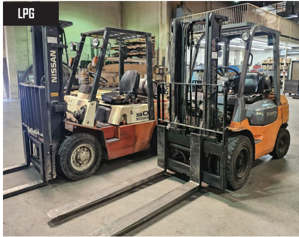
Nissan Optima 50 5000# Capacity LPG Forklift, 3 Stage Mast, Side Shift, 48" Forks, Yard Cushion Tires, S/N 257H and Toyota 7FGU30 6000# Capacity LPG Forklift, 2 Stage Mast, Side Shift, 60" forks, Yard Cushion Tires, S/N 62379
