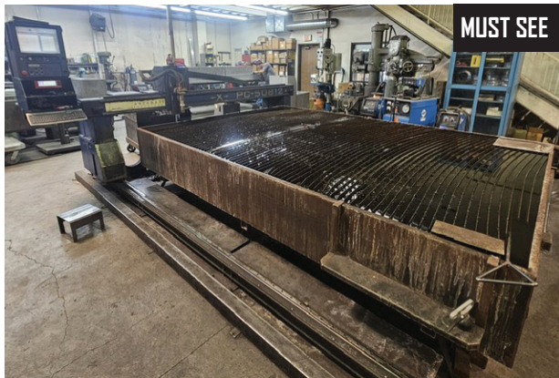
Axis PC-50812 CNC Plasma Cutting System, 12' X 9" Table, Kalburn Sprirt 275A 150 Volt 275 Amp Plasma Cutting and Marking System S/N 1240408, Promotion CNC Control, 1 Cutting Head
