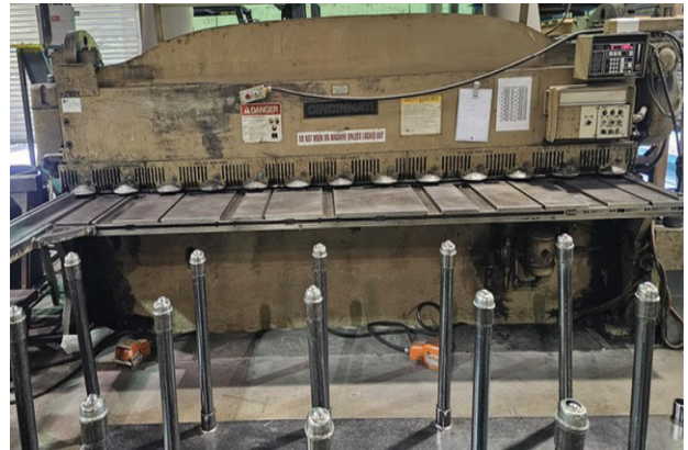
Cincinnati 1812G Mechanical Shear, 12' X 1/4" Capacity, 48" Front Operated Backgauge, Microcomputer Gauge Control, 60 Strokes/Minute, 13 Hold Downs, S/N 48294.
