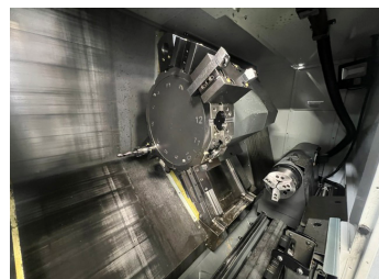
2023 HAAS ST-30Y CNC Turning Center w/ C & Y Axis, 12 Station Live Tool Turret, 10" Chuck, 3" Bar Capacity, 3400 RPM, Chip Conveyor and Haas Barfeeder -V2-
