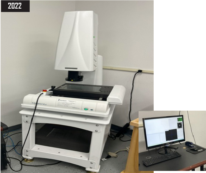
2022 Micro-Vu Vertex 261 Multisensor Vision Measuring Machine (VMM), 250 mm x 160 mm x 160 mm (XYZ), w/ Inspec Software, s/n M2840U0001.
