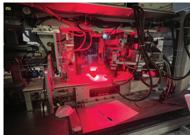
2016 Komax Xcell 3000 Stringer High Efficiency Solar Cell Production Machine w/ Allen Bradley Panel View Controls.
