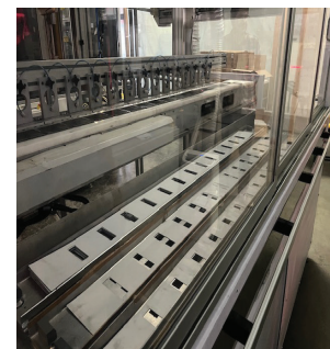
2016 Komax Xcell 3000 Stringer High Efficiency Solar Cell Production Machine w/ Allen Bradley Panel View Controls.
