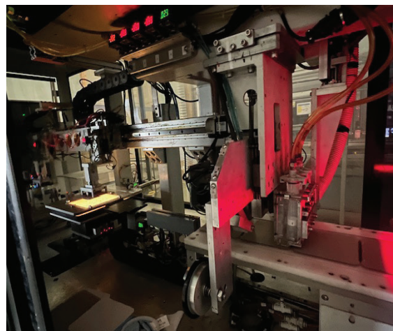
2016 Komax Xcell 3000 Stringer High Efficiency Solar Cell Production Machine w/ Allen Bradley Panel View Controls.
