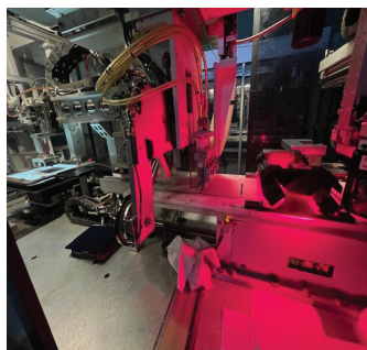
2016 Komax Xcell 3000 Stringer High Efficiency Solar Cell Production Machine w/ Allen Bradley Panel View Controls.
