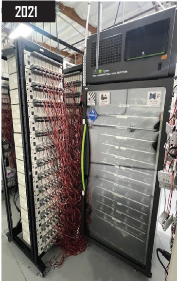
2021 Neware 14 Module Battery Test System model 425W CT4008T-5V6A-S1 and Caron 60401 Refrigerated Incubator.
