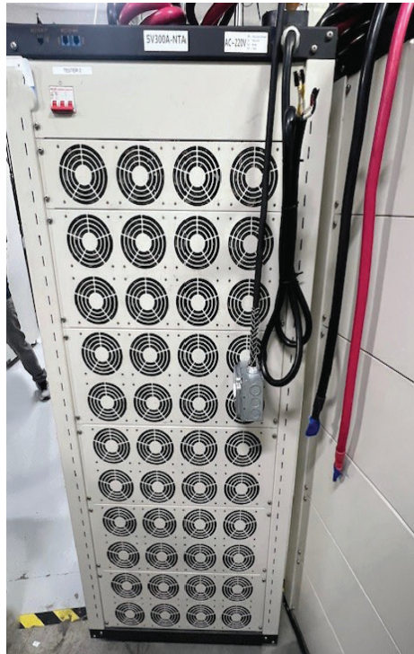
Neware 5V300A-NTA Battery Test System.
