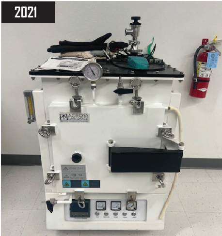
2021 Across Atmosphere Muffle Furnace model GCF1200-12X8X8,
