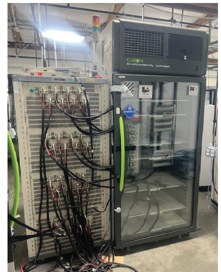
Neware 4 Module Battery Test System model and Caron 6021-1 Refrigerated Incubator.
