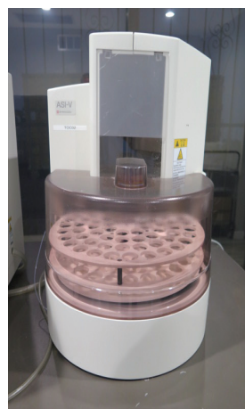
SHIMADZU TOC-VWP TOTAL ORGANIC COMPOUND ANALYZER W/ SHIMADZU ASI-V AUTOMATIC SAMPLER
