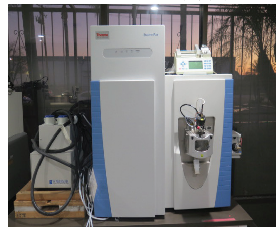
THERMO SCIENTIFIC EXACTIVE PLUS HYBRID QUADRUPOLE-ORBITRAP MASS SPECTROMETER W/ VACUUM PUMP AND PUMP
