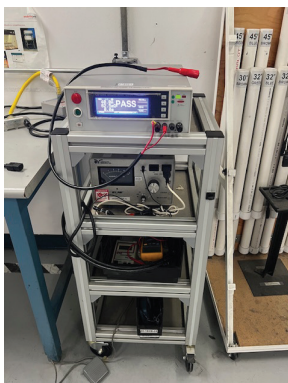
Partial View of Test Equipment
