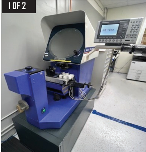
Mitutoyo PH-A14 14" Optical Comparator s/n 008921211 w/ Heidenhain Quadra-Chek Programmable DRO, Surface and Profile Illumination, Holding Fixtures, 20X and 50X Lens Sets, Cabinet Base.
