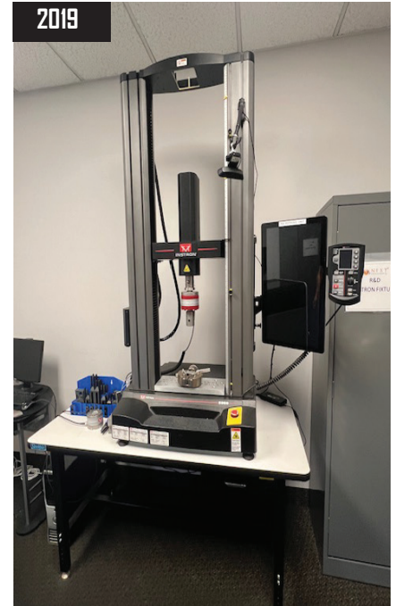
2019 Instron 5966 Config E1-F1-G1 10kN Digital Universal testing System s/n 5966B19163 w/ Instron Digital Controls, 10kN Head, Grip Clamp and Rigid Hold Toolin
