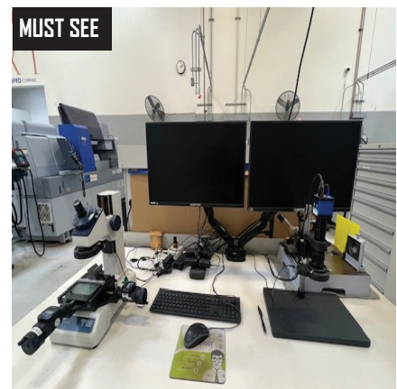
Mitutoyo TM Tool Makers Microscope s/n 100412109 w/ Digital Micrometer Head and Light and Hayear Video Inspection Scope w/ Monitor.
