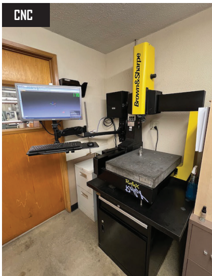
Brown & Sharpe Reflex Model 343 CMM, w/ CMM Manager Software and upgrades.
