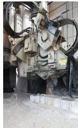
Cincinnati Milacron 30V Bridge Profiler 5-Axis CNC Bridge Mill w/ Siemens Acromatic 950 Controls, 50-Taper Spindle, 30Hp
