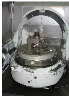
2012 Mori Seiki NMV-5000 DCG HSC 5-Axis CNC VMC w/ Mori F31iA5 Controls, 120-ATC, CAT-40, 18,000 RPM, 20" Rotary
