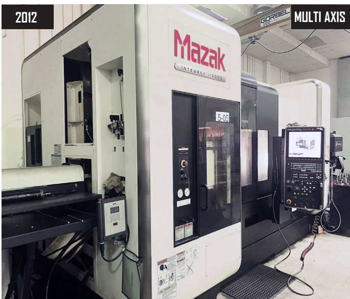
2012 Mazak Integrex i-300S Intelligent /Multi-Tasking Twin Spindle CNC Turning Center w/ Mazatrol Matrix 2 Controls, 120-ATC, Capto C6, "Y" Axis, "B" Axis Live Tooling, 4000 Main and Sub Spindle RPM, 12,000 Milling RPM
