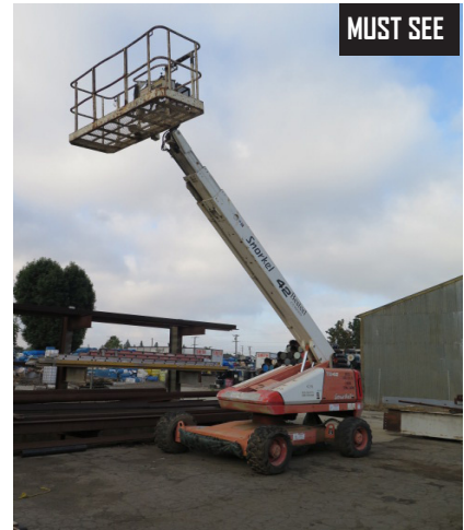
2007 Snorkel TB42CU Boom Basket Lift s/n JA07146 w/ Diesel Engine, 500 Lb Cap, 42' Max Boom Height, 33' Platform Reach, 30" x 92" Basket.
