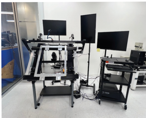
Optical System with Canon Camera and Table.
