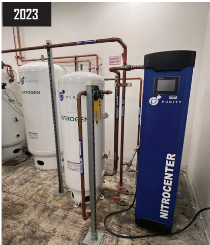
2023 Purity PGN2-L4 Nitrogen Generator with Tanks.
