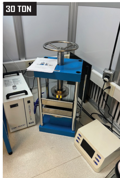
MSE Pro 30 Ton Heated Lab Press.
