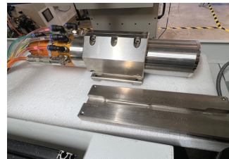
2023 Ametek Nanoform 700 Ultra A21200-01 REV. H Multi Axis Precision Machining System, For Production of Optical lenses, Mirrors and Mechanical Components, 80,000 RPM Spindle Head, 700mm Swing and 170kg Load Capacity, Video System, Surface Finish of 1nm Ra, 350x mm and 300z Travel Oil Hydrostatic Machine Slides, Ametek Cooling System, FTS5000 Diamond Holder.
