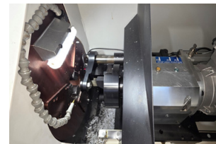
JF Berns Servo Auto Champ 2 Chamfer Machine, model SAC2, s/n SAC201-175.
