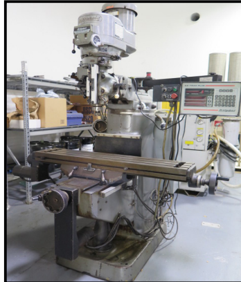
Bridgeport / Ez-Trak 2-Axis CNC Vertical Mill s/n BR254862 w/ Bridgeport EZ-Trak Plus Controls, 60-4200 Dial-Change RPM, Kwik-Switch Taper Spindle, Chrome Ways, 9" x 42" Table.
