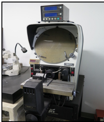
Gage Master R-14 14" Optical Comparator w/ Quick-Chek DRO, Surface and Profile Illumination, Stand.
