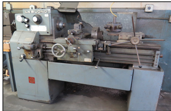
LeBlond Regal 15" x 36" Lathe w/ 45-1800 Servo Shift Dial RPM, Inch Threading, 6-Station Turret Assy, Tool Post, Trava-Dial, 5C Collet Closer, Coolant.
