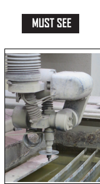
Omax 80160 5-Axis CNC Waterjet Contour Machine s/n E511599 w/ Omax CNC Controls, 6' x 12' Sheet Cap, Tilt-A-Jet 5-Axis Cutting Head, mdl. 4055V 40Hp 55,000 PSI Pump, Koolant Koolers Cooling Unit.
