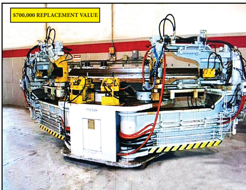
Cyril Bath CNC Stretch Wrap Forming Machine Modle V-20, Tension Pull 20 Ton Located in City of Industry CA.
