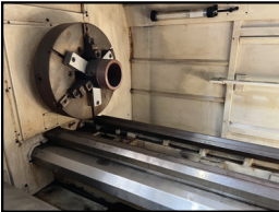
Summit "Smart Cut" SC30-9X80M Big Bore CNC Turning Center w/ Fagor Controls, 9" Thru Spindle Bore, 4-600 RPM, 8-Station Turret, Tailstock, (2) 24" 3-Jaw Chucks
