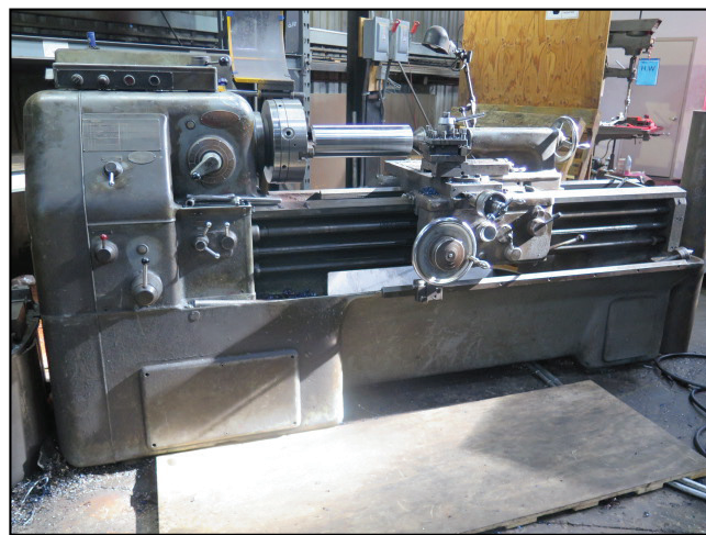
Okuma LS 18" x 54" Geared Head - Gap Lathe w/ 35-1800 RPM, Inch Threading, Tailstock, Tool Post, 12" Chuck
