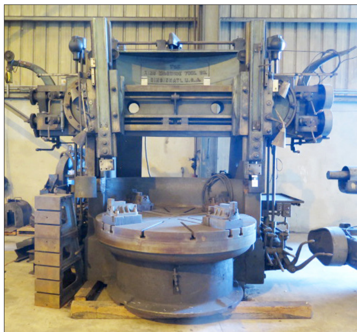
KING VERTICAL BORING MILL VIEW LOT #14
