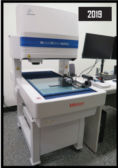
2019 Mitutoyo "Quick Vision Active" mdl. QVT1-L404ZiL-D Video CMM Machine
