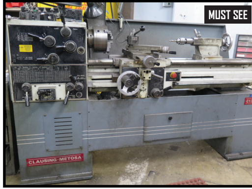
Clausing Metosa C1340S 13" x 40" Geared Head Gap Bed Lathe w/ Anilam DRO, 75-2500 RPM, Inch/mm Threading, Tailstock, 8" Chuck
