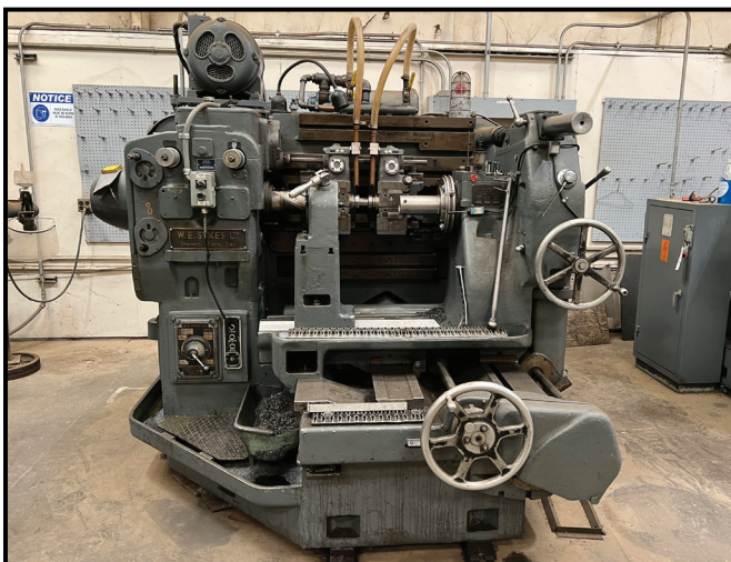
W.E. SYKES MODEL C.S.2 HARRINGBONE GEAR GENERATOR, 25" MAX BLANK DIAMETER GEAR.
