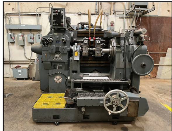
W.E. SYKES MODEL 3C DOUBLE HELICAL, HARRINGBONE GEAR GENERATOR.
