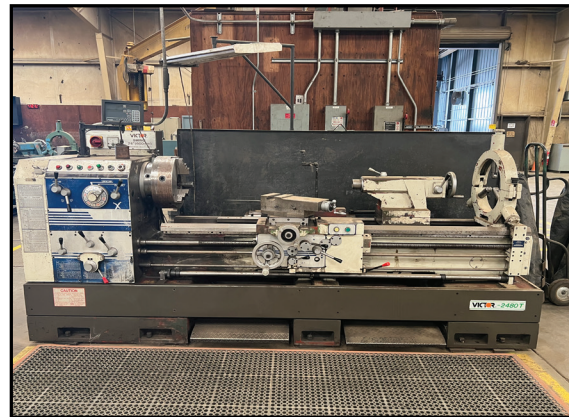
VICTOR 2480T, 24" X 80" GAP ENGINE LATHE, 4" THROUGH HOLE, 25 TO 860 RPM, 16" 3 JAW CHUCK, NEWALL DRO, IN/METRIC THREADING, TAPER ATTACHEMENT.
