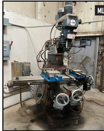
LAGUN REPUBLIC B-40 VERTICAL MILLING MACHINE WITH 3 POWER FEED TABLES, DRO.
