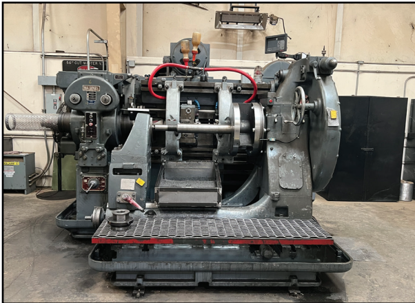
W.E. SYKES TYPE CS-2 HARRINGBONE GEAR GENERATOR.
