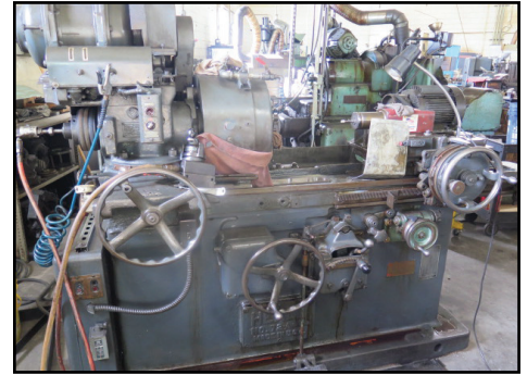
Heald 72-A ID Grinder w/ Motorized Work Head, 6" 3-Jaw Chuck, Red Head Grinding Head
