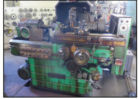
Ex-Cell-O Style 33 6" x 16" Thread Grinding Machine w/ Work Head, Tailstock
