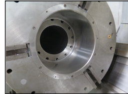
1997 Mori Seiki SL-80 Big Bore CNC Turning Center w/ Mori Seiki SC-518 Controls, 10 1/2" Thru Spindle Bore, 6-Station Turret, 4-550 RPM, 33" 3-Jaw Chuck with 16" Bore
