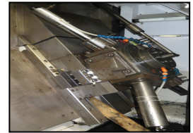
1997 Mori Seiki SL-80 Big Bore CNC Turning Center w/ Mori Seiki SC-518 Controls, 10 1/2" Thru Spindle Bore, 6-Station Turret, 4-550 RPM, 33" 3-Jaw Chuck with 16" Bore
