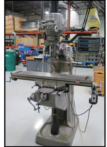
Bridgeport Vertical Mill w/ Acu-Rite MillMate DRO, 2Hp, 60-4200 Dial RPM, Kurt Power Draw-Bar, Chrome Ways, Power Feed
