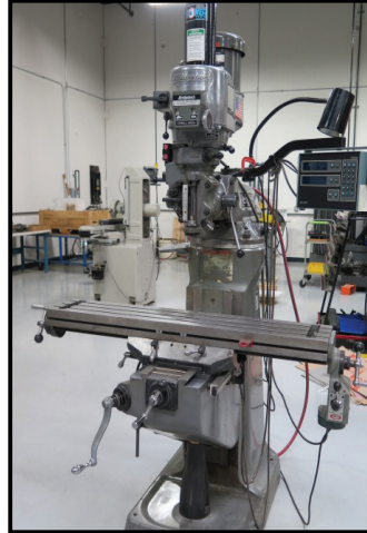
Bridgeport Vertical Mill w/ Acu-Rite MillMate DRO, 2Hp, 60-4200 Dial RPM, Kurt Power Draw-Bar, Chrome Ways, Power Feed
