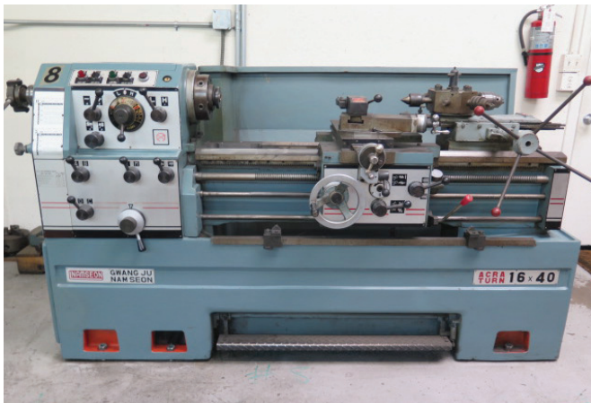
Acra Turn 16" x 40" Gear-Gap Lathe w/ 33-1800 RPM, Inch/mm Threading, Tailstock, Steady Rest, 6-Station Turret, 8" 3-Jaw Chuck, 5C
