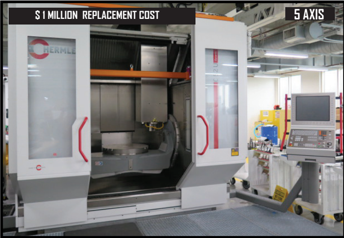
2015 Hermle "C52U Dynamic" 5-Axis Machining Center s/n 23959 w/ Hermle / Heidenhain Controls, Laser Tool Presetter, 60-Station ATC Plus 153 Station Tooling Tower, HSK63 Spindle, 700mm (27.56") Rotary Rable, +100 Degree / -130 Degree Swivel Range, Travels X=1000mm (39.37"), Y=1100mm (43.3"), Z= 750mm (29.52"), Hyfra Pedia VWK70-DE-J Cooling Unit s/n 15040605, Knoll Handt KSS-Abscheider EM-DS 1-0,5NF High Pressure Coolant and Filtration System, Chip Conveyor.
