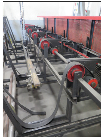
2004 Amada SA90A Rotary Pipe Cutter s/n 90000005 w/ Amada Controls, Automatic Pipe Loader, 1.25"-3.54" x .24" Max Pipe Dia., 137.8"-255.6" Max Pipe Length, 1 ¼", 1 ½", 1 ¾", 2", 2 1/8", 2 ¼", 2 ½" and 3" Collet and Liner Sets.
