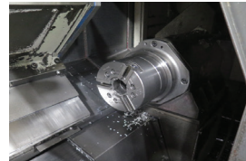
2001 Mazak Super Quick Turn 200MS Live Turret – Twin Spindle CNC Turning Center s/n 152105 w/ Mazatrol 640T PC-FUSION-CNC Controls, Tool Presetter, 12-Station Live Turret (NO TOOLING), 8” 3-Jaw Main Power Chuck, 6” 2-Jaw Sub Spindle Power Chuck, Chip Conveyor, Coolant.
