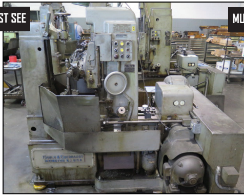
Goule & Eberhardt 12H Universal Gear Hobbing Machine w/ 18" Table
