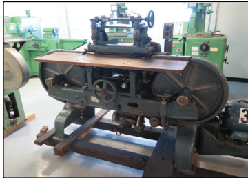
Hudson General USM mdl. A 12' Leather Splitting / Thinning Saw
