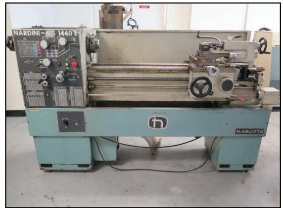
Nardini MS1440E "Mascote" 14" x 40" Geared Head Lathe
