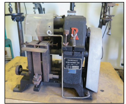
Randall NSB Leather Belt Beveling Machine
