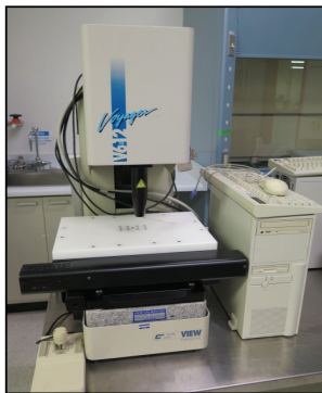
1999 View Engineering "Voyager X6X12" Non-Contact CMM Machine w/ Joystick Controller
