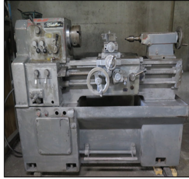
Cadillac 13" x 24" Geared Head Gap Bed Lathe w/ 83-1800 RPM, Inch Threading, Tailstock, 6"Chuck
