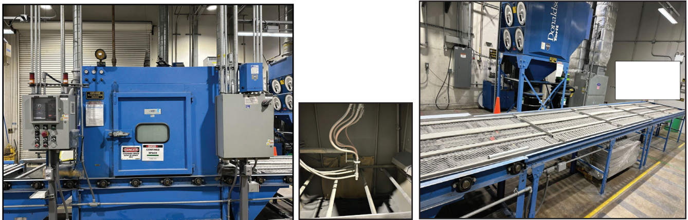
ICM ABRASIVE CONVEYORIZED SAND BLASTER MODEL G43430 WITH DONALDSON TORIT MODEL DFO 2-9 DUST COLLECTION SYSTEM, CONTROLS AND SUPPORT.
