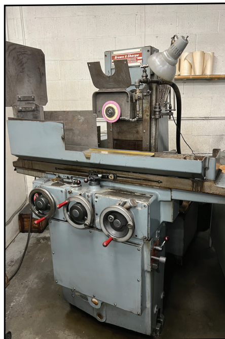
BROWN & SHARPE 618 ICRMASTER SUFRACE GRINDER.
