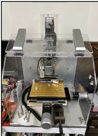
CAMERON MODEL 2001-S CNC MICRO MILLING MACHINE WITH COMPUTER.
