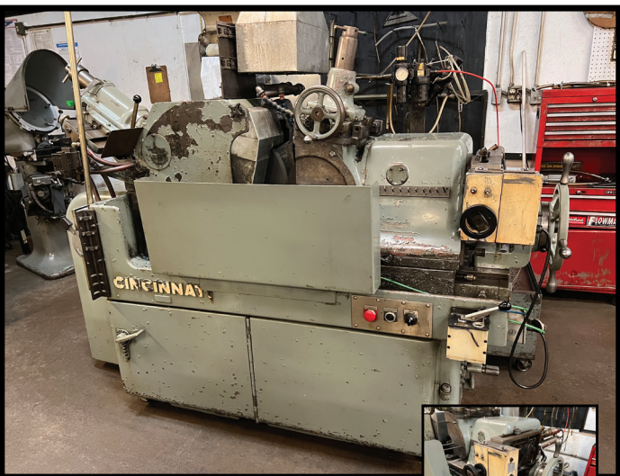
CINCINNATI MODEL OM CENTERLESS GRINDER, 24" WHEEL, W/ ALLEN AIR BELLOWS END FEED ATTACHMENT.
