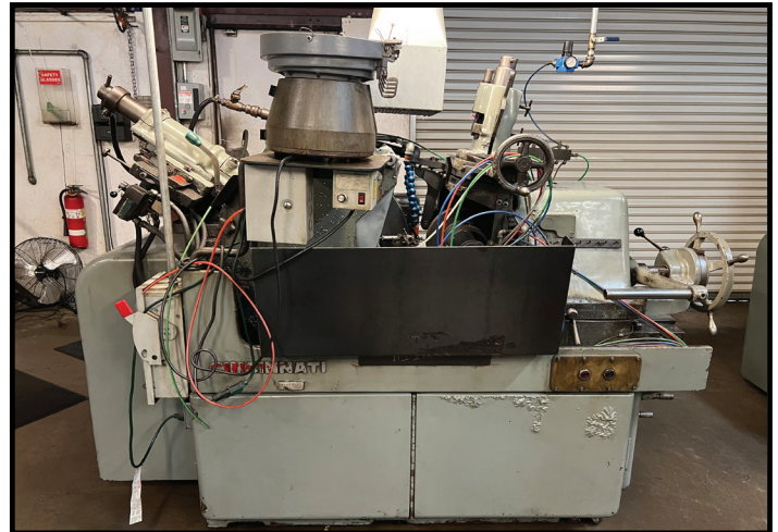
CINCINNATI MODEL OM CENTERLESS GRINDER, 24" WHEEL, S/N 2M2H1W-29.
