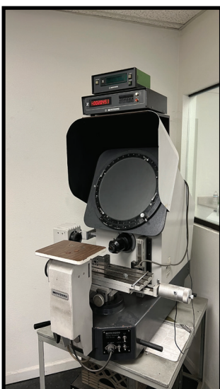
MITUTOYO PH-350, 14" OPTICAL COMPARATOR WITH DRO.
