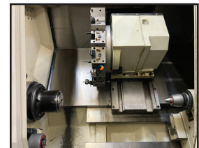
DAEWOO PUMA 250B CNC LATHE, W/ MITSUBISHI CONTROL, 12 POSITION TURRET, 3" THRU HOLE, TAIL STOCK, 10" CHUCK, S-30 COLLET NOSE, CHIP CONVEYOR, SMW SPACESAVER 2003 BAR FEEDER
