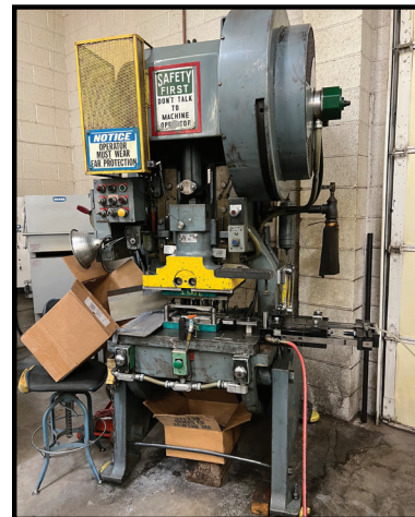
L & J MODEL W27, 27 TON OBI PUNCH PRESS, 2.5" STROKE, 32" X 16.5" TABLE.
