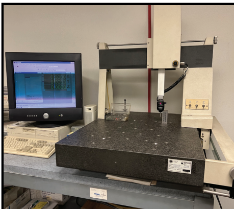
NUMEREX CMM WITH 3D WORKSHOP SOFTWARE AND RENISHAW MIP PROBE SYSTEM
