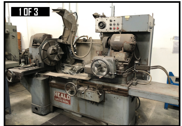
1 OF 3) HEALD MODEL 273A UNIVERSAL I.D. GRINDER, S/N 43605.
