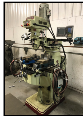
2007 ACER VERTICAL MILLING MACHINE W/ ACU-RITE DRO, POWER FEED, VARIABLE SPEED.
