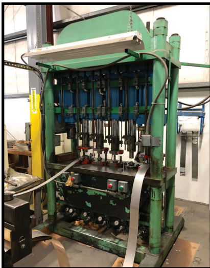
HYDRAULIC CONTINUOUS STAMPING PRESS W/ 6 VERTICAL HEADS, AND UNCOILERS.
