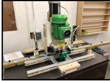
GRASS ECO PRESS-P HINGE BORING MACHINE.
