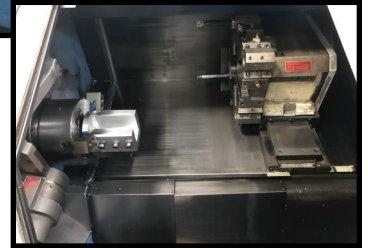
MAZAK MODEL QT20N CNC LATHE, WITH FANUC 10T CONTROL, 8" CHUCK, TAIL STOCK.
