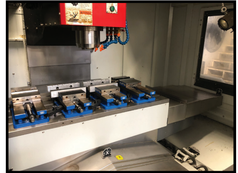
2015 YAMA SEIKI AWEA AV-1060 CNC VMC, W/ 15,000 RPM, CAT 40, 30 ATC, FANUC Oi-MF CONTROL, 2455 RUN TIME, 3 AXIS, (XYZ) 41.7" X 23.6" X 23.6", S/N 1060-15059.
