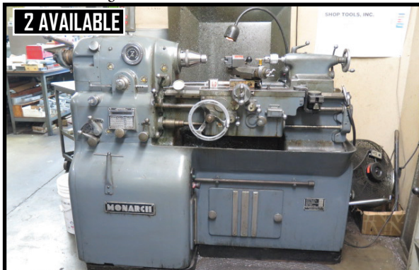
Monarch 10"EE 12 1/2" x 20" Lathe w/ Newall DRO, 3000 RPM, Inch Threading, Tailstock, 5C, KDK Tool Post ***2-AVAILABLE*** Threading, Tailstock, Trava-Dial, 5C, KDK Tool Post
