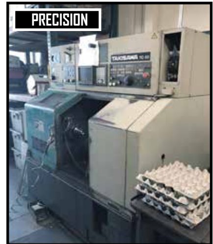
Takisawa TC-30 CNC Turning Center w/ Takisawa -Fanuc Controls
