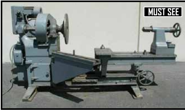
Prybil L-28-23 27" x 60" Cap. Gap Bed Spinning Lathe
