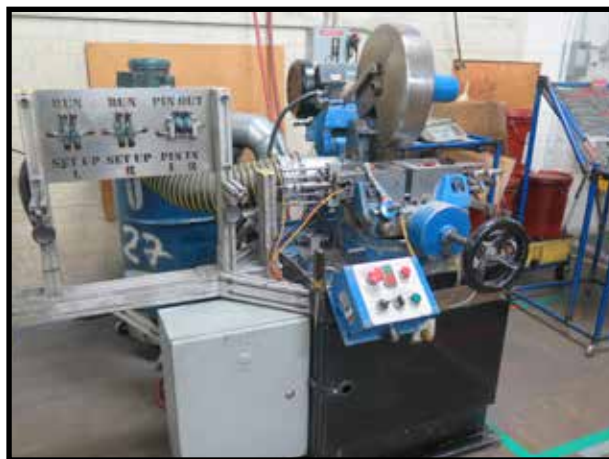
Kalamazoo FA350SA Miter Cold Saw
