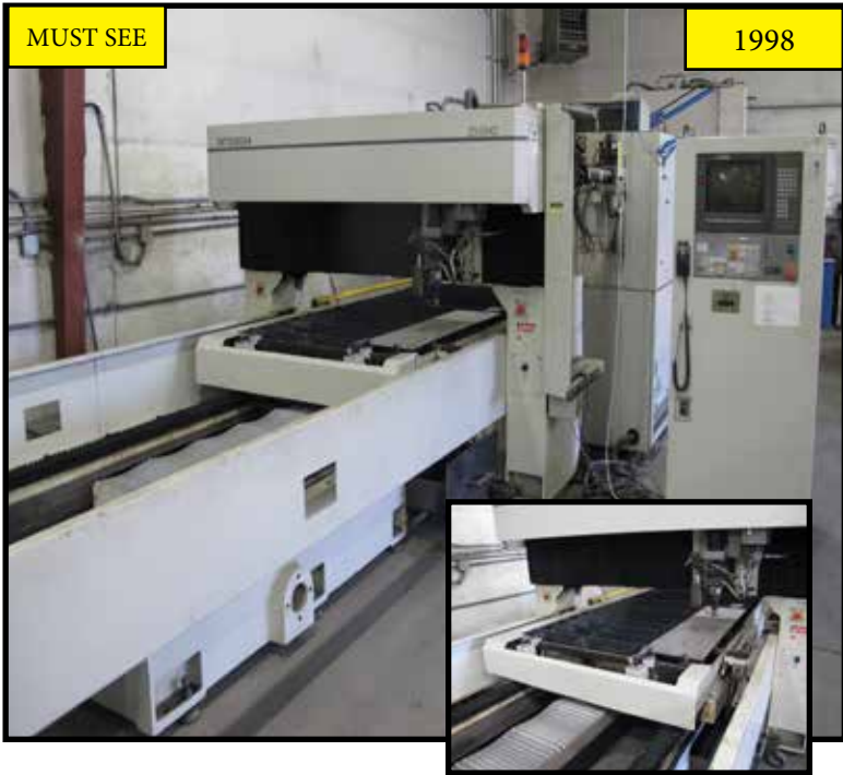
MUST SEE 1998 1998 MITSUBISHI ML 2512-HD 3000 WATT CO2 CNC LASER CUTTING MACHINE, W/4FT X 8FT TABLE, LC10BV CONTROL, (2600 mm X 1250 mm X150 mm) (XYZ), S/N 68251HD238.
