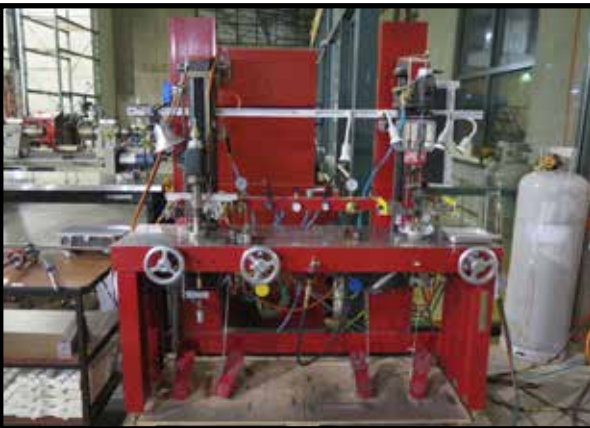
2-Station Glass Tube Pinch Press w/ Rotary Die Heads
