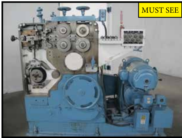
Torrington mdl. W12-A Precision Coil Spring Winder w/ 0.047-0.148 Wire Cap, ¼"-2 ¾" Coil OD Range, Straightener
