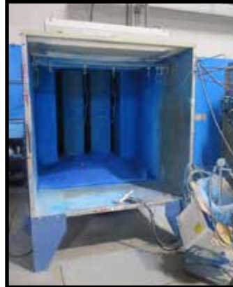
Nordson "Econo-Coat" NVC4 5' x 5' x 5' Powder Paint Booth
