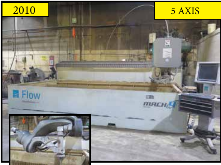
2010 Flow MACH4 4020b mdl. 044917 5-Axis Dynamic XD CNC Waterjet Contour Machine
